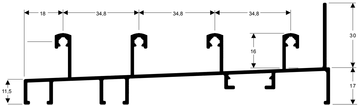
TMS-122 1,401 kg/m
