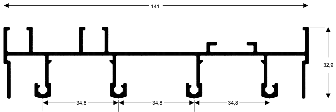
TMS-121 1,449 kg/m
