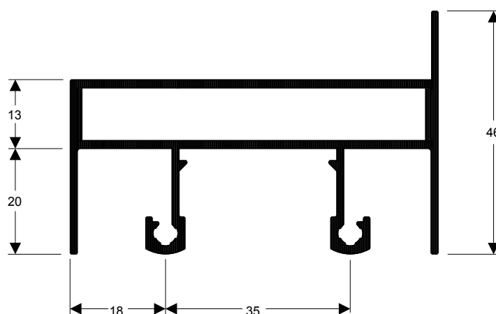
TMS-005 1,058 kg/m
